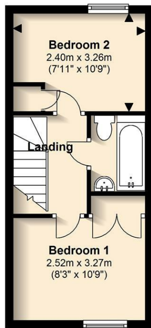
First Floor Approx. 24.7 sq. metres (265.4 sq. feet)
